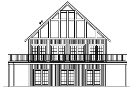
REAR ELEVATION (LAKE SIDE)
