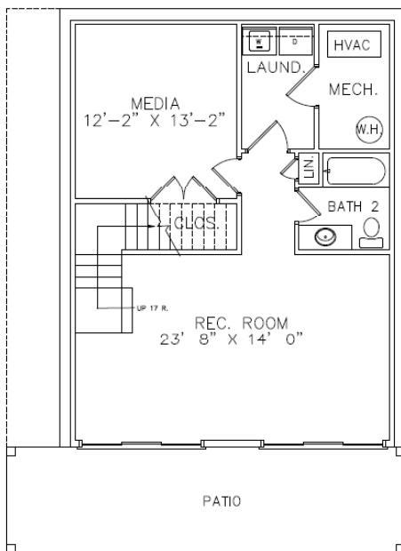
LOWER LEVEL FLOOR PLAN
